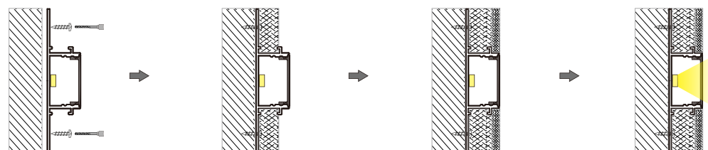
LED Aluminum heat dissipater (H.D.)
