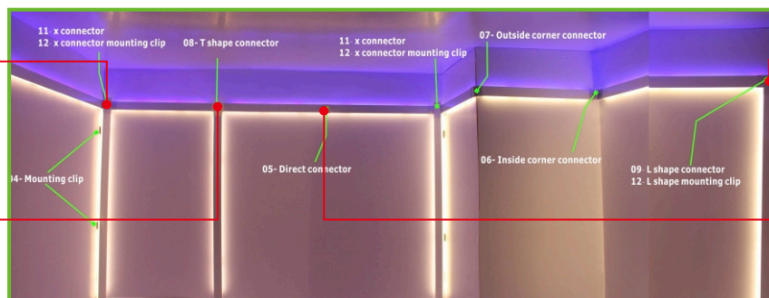
X-shape Connector
